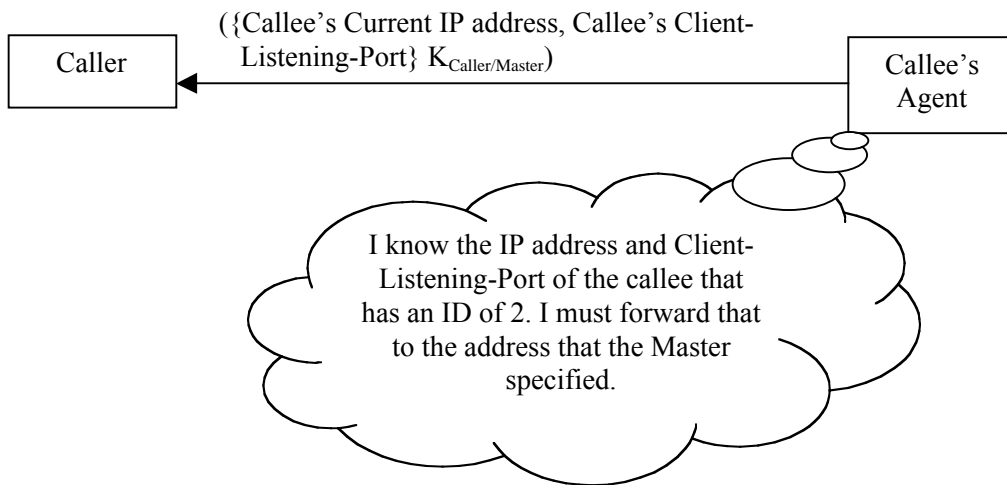
Step 4: Callee's Agent sends the Caller, Callee's IP and port
