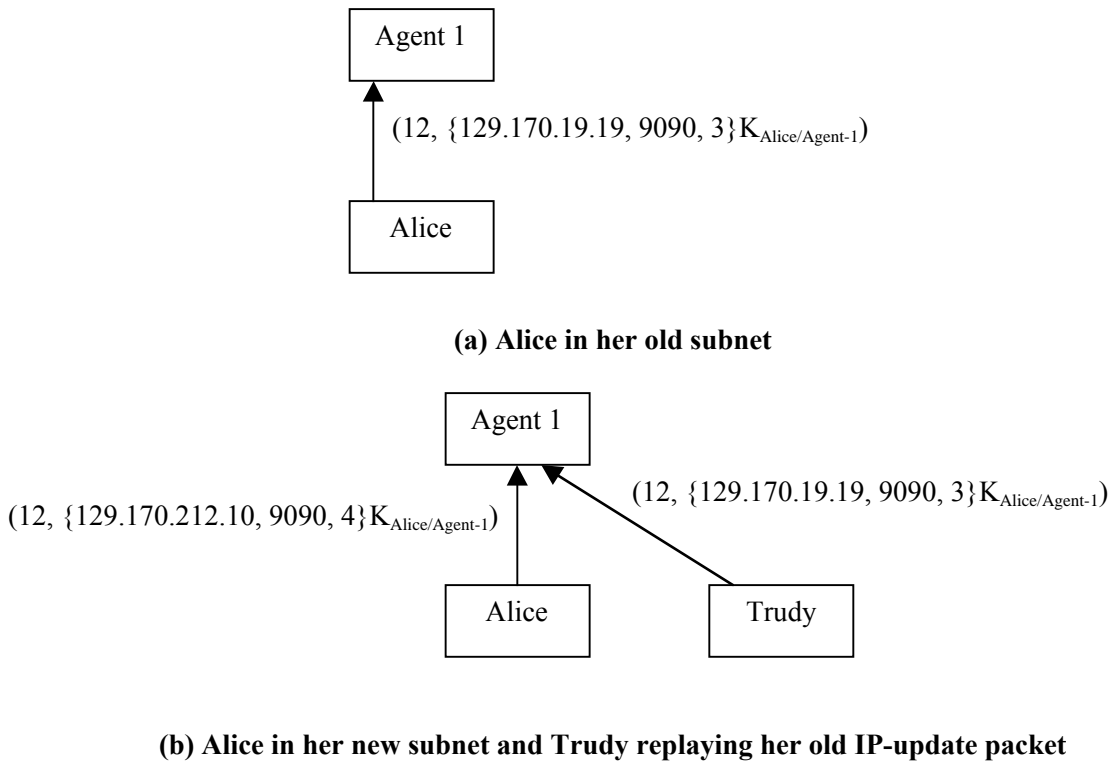
Figure 13: An impostor replaying an old subnet packet after a Client switches Subnets
