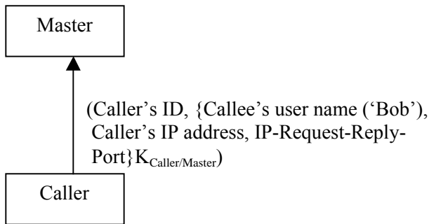
Step 1: Caller sends an IP-request to the Master
