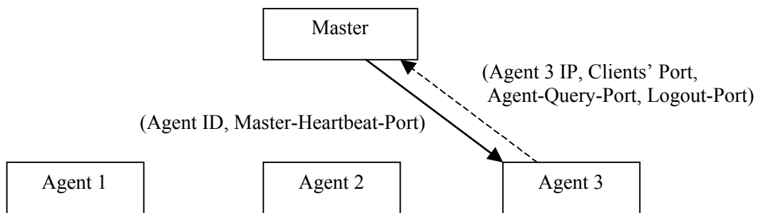
Figure 2: An Agent (Agent 3) registering with Master
