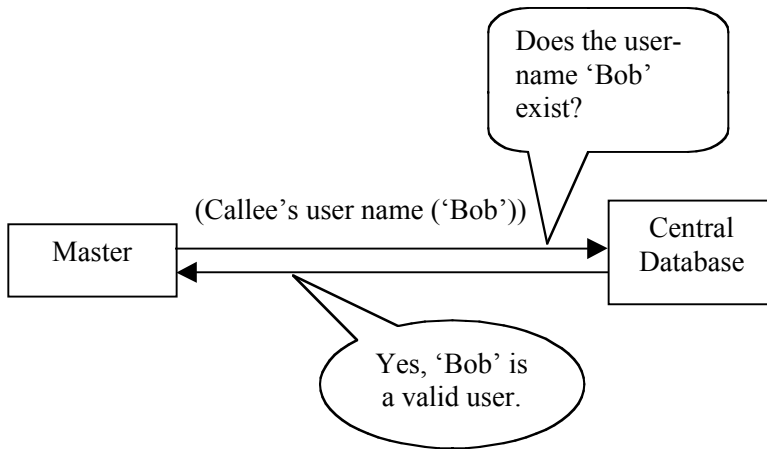
Step 2: The Master queries the Database for the validity of the Callee
