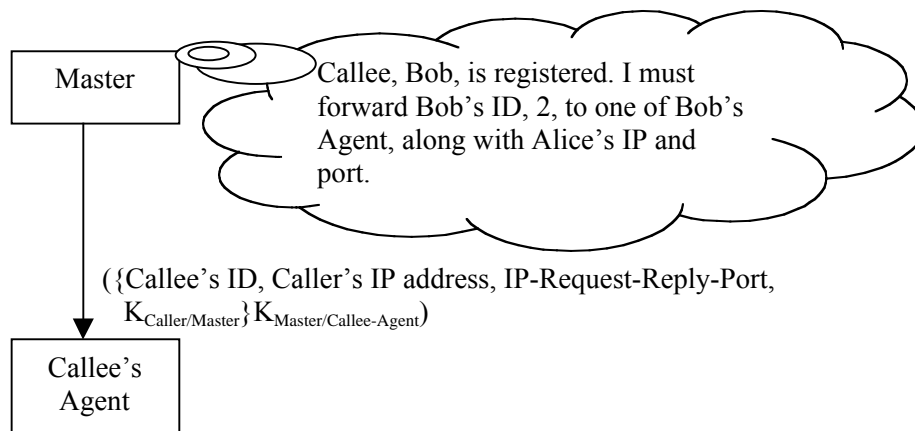
Step 3: The Master forwards the IP-request to one of Callee's Agent
