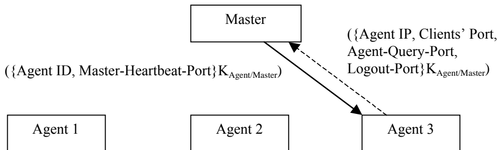
Figure 9: Agent registering with Master using Encryption
