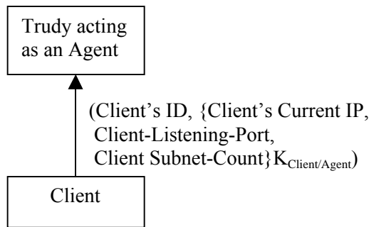
Figure 16: Impostor acting as an Agent
