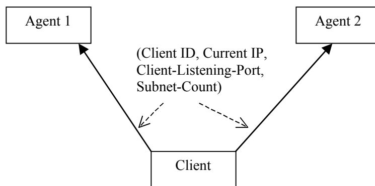
Figure 7: A Client updating its IP with two Agents
