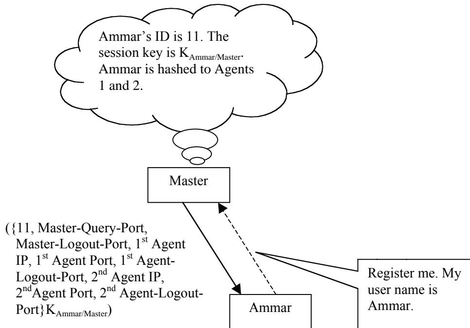
Figure 10: A successful Client registration with Encryption
