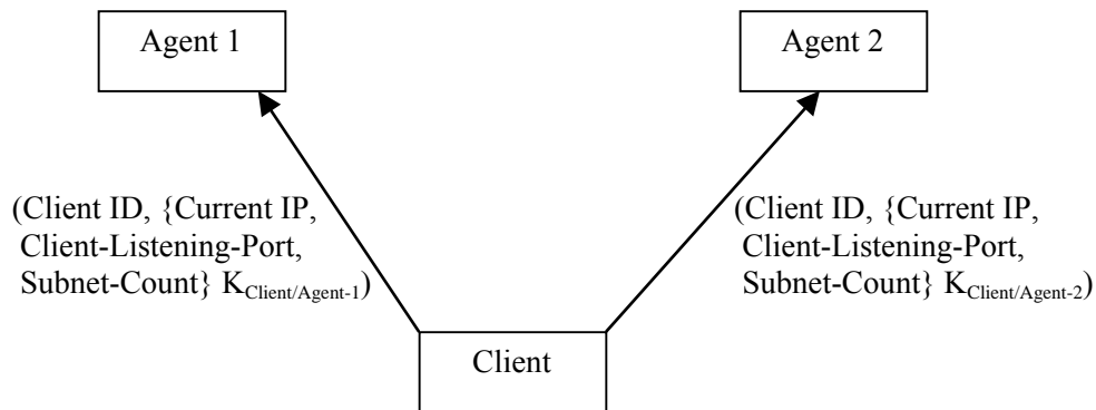
Figure 11: A Client updating its IP with its Agents using Encryption
