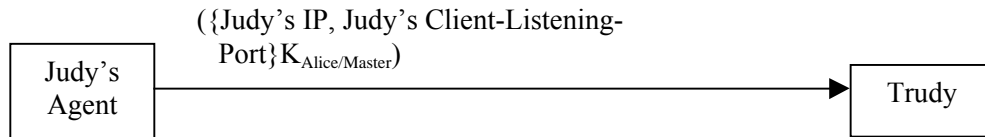
Figure 15: Impostor obtaining an IP address by a replay attack
