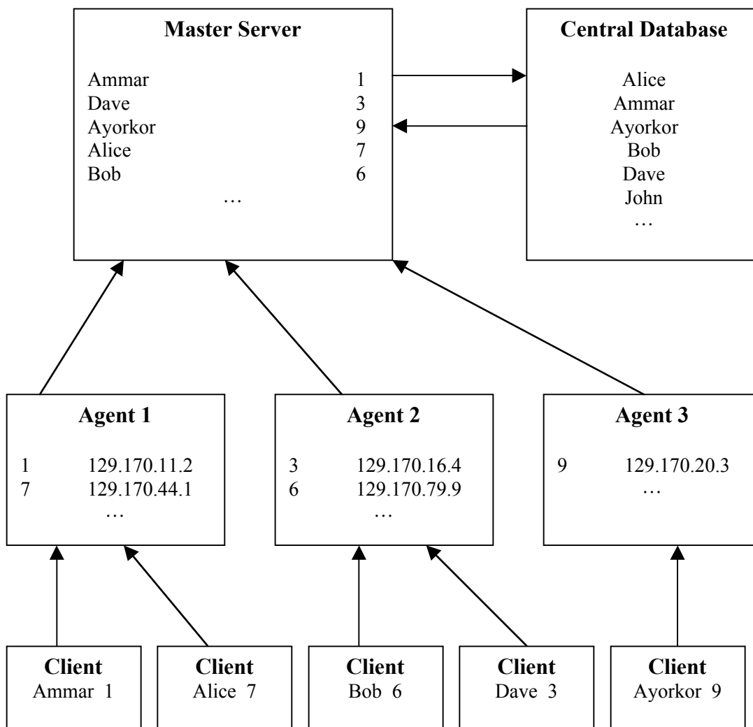
Figure 1: Layout of Directory
