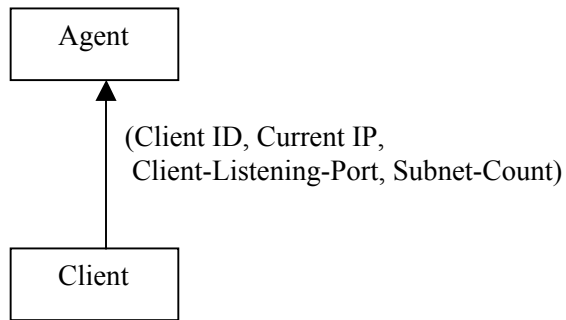
Figure 4: Client sending IP-update packet
