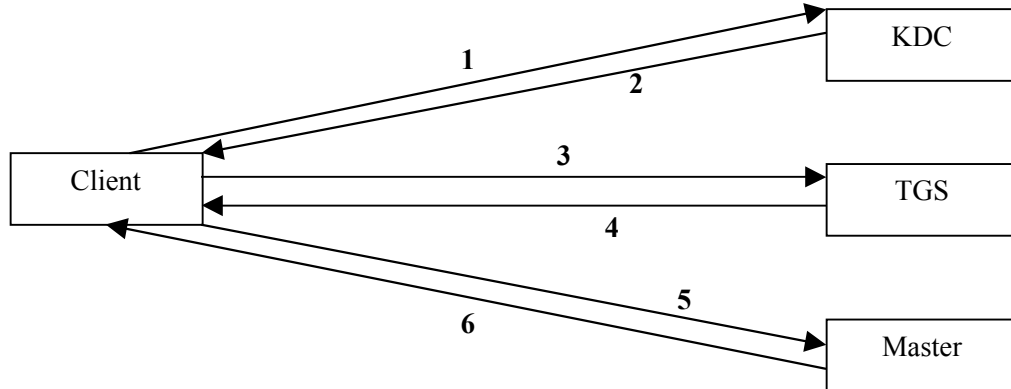
Figure 8: Kerberos Authentication Process before a Client/Agent registers
