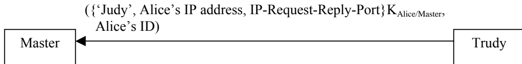
Figure 14: Impostor conducting a replay attack to obtain an IP address
