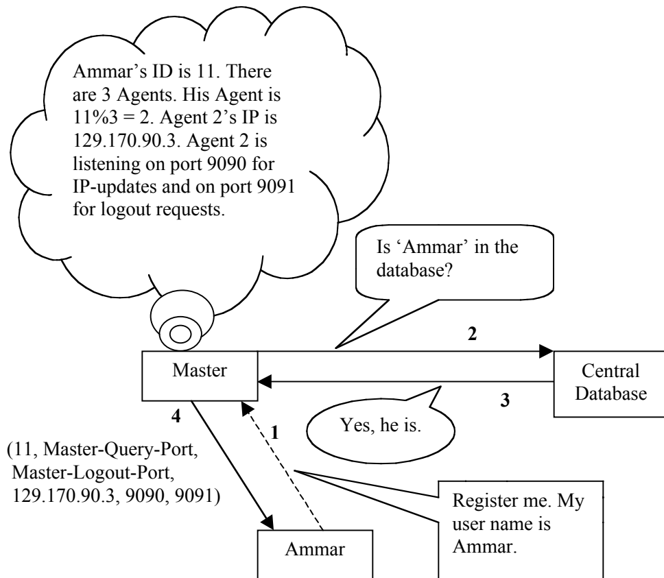
Figure 3: The Client registration process
