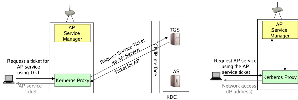
(b) Requesting the AP service ticket
